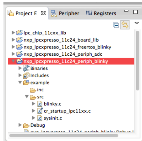
Figure 4: Pick project
