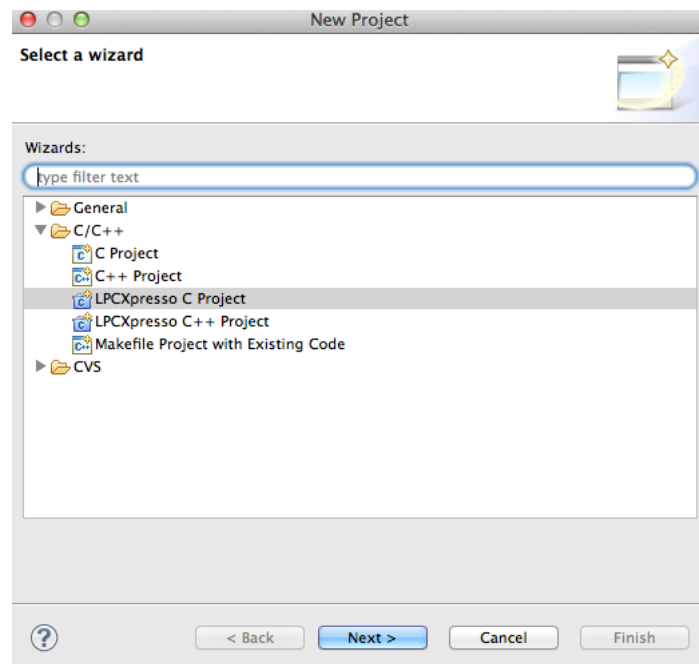
Figure 8: New Project
