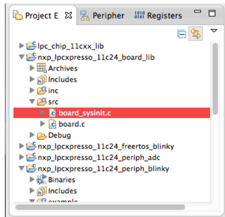
Figure 7: board_sysinit.c
