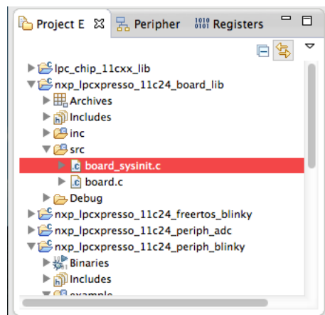
Figure 7: board_sysinit.c
