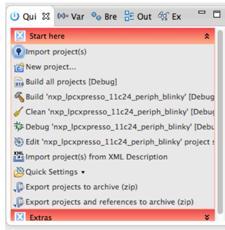
Figure 6: First Build
