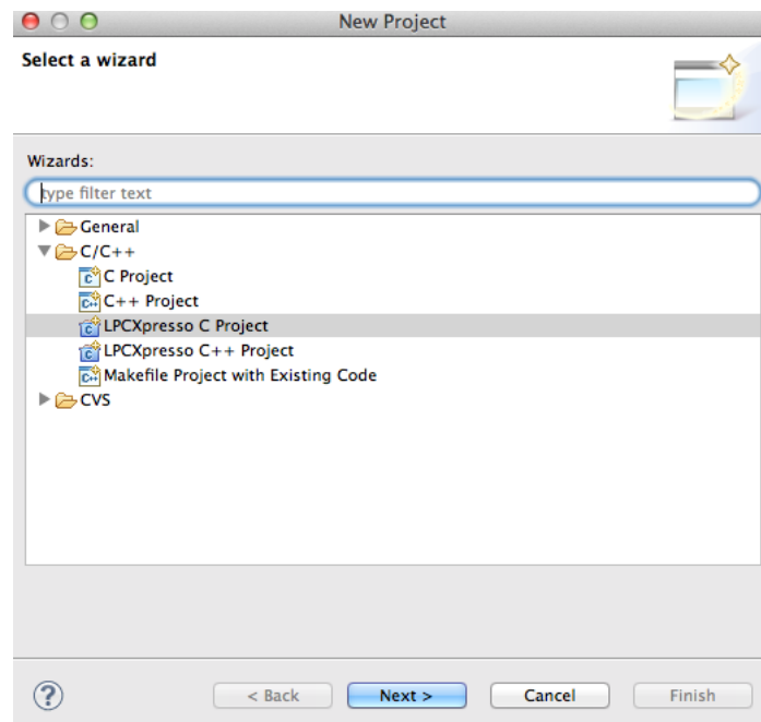
Figure 8: New Project
